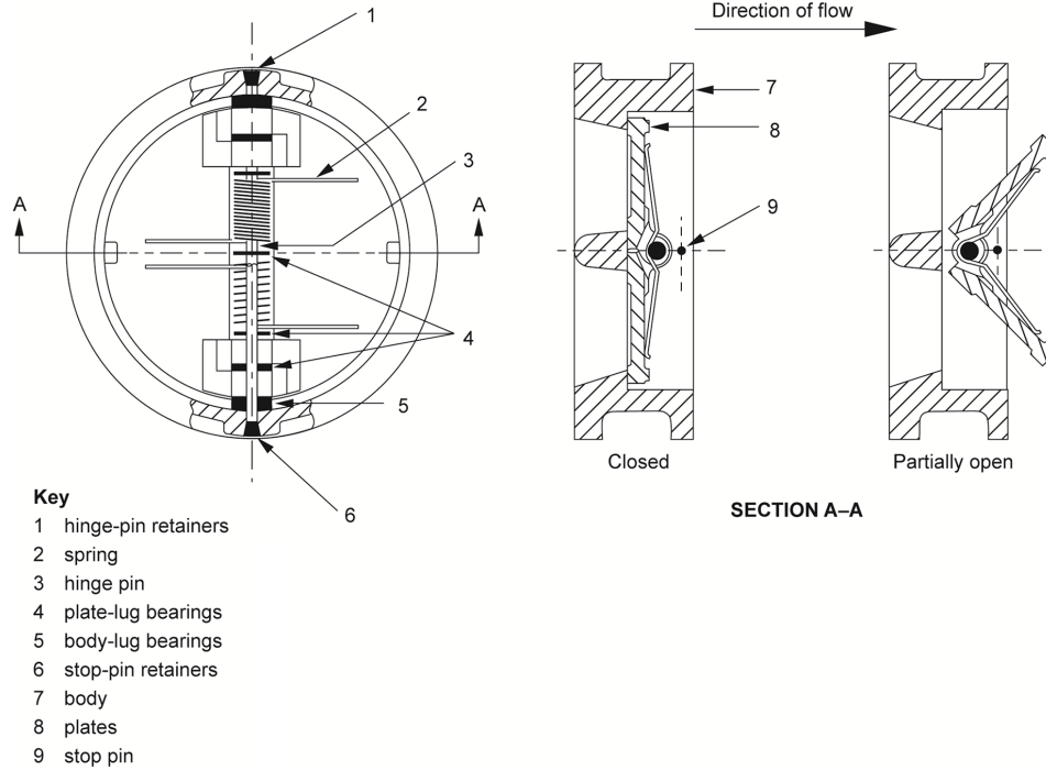
Figure 7—Cross Sections of Typical Check Valves ( continued )
